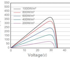
Power Voltage Curve SP360M/60
